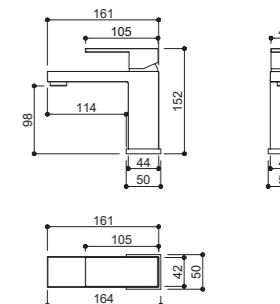
Ref. KR225NB Acabamento black matte [1367].
