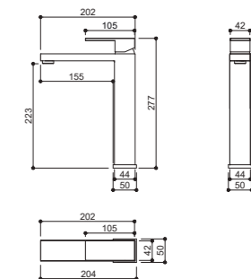
Ref. KR229NB Acabamento black matte [1368].
